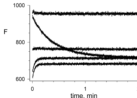
FIGURE 2: Reactions of carbachol with AChE monitored by thioflavin T fluorescence. Reactions were initiated by stopped-flow mixing of AChE with carbachol and thioflavin T as outlined in the Experimental Procedures, and the fluorescence F was recorded continuously. Initial concentrations of thioflavin T ( 15.6 \mu\text{M} ) and AChE ( 152 \text{ nM} ) were the same in each reaction, while the respective concentrations of carbachol were 0, 0.5, 10, 40, and 60 mM (from the upper to the lower trace taken at time t = 0 ). F_B (eq 5) from the components individually was 83.
