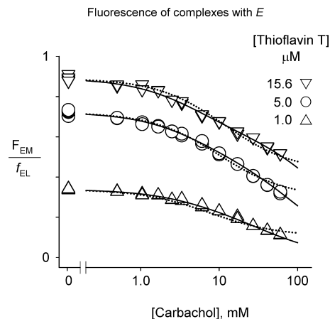
FIGURE 4: Determination of carbachol binding constants with free AChE from the initial fluorescence of AChE-bound thioflavin T (23). F_{EM} values from mixtures of AChE (70–155 nM), thioflavin T (1.0–15.6 \mu\text{M} , as noted), and the indicated concentration of carbachol were determined from stopped-flow traces as in Figure 3. The F_{EM} data from each set at fixed thioflavin T concentration were fitted initially to eq 10 to obtain f_{EL} for the set, and F_{EM}/f_{EL} from all three sets were then analyzed simultaneously with eq 10 as described in Experimental Procedures. Parameters obtained from the data fitting are shown in Table 1. The dotted lines show the one-site fit when carbachol is assumed to have no affinity for the P-site ( (iK_S)^{-1} fixed at 0) with fitted parameters K_{M+S} = 6.2 , f_{EL}/f_{ESL} = 1.85 , and i_2 = 2.1 .
