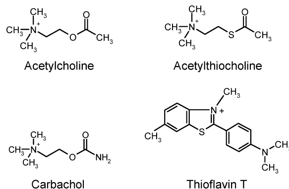
FIGURE 1: Structures of acetylcholine analogues and thioflavin T.
