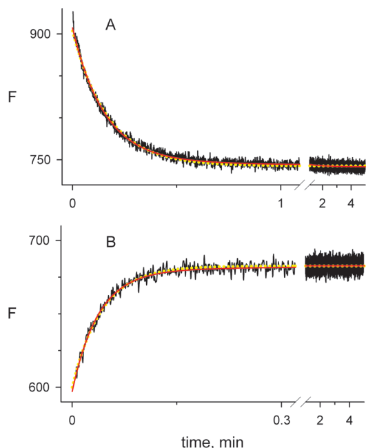
FIGURE 3: Analysis of reactions of carbachol with AChE. Reaction traces were obtained in the presence of thioflavin T under the conditions in Figure 2 with 1.67 mM carbachol in panel A or 60 mM carbachol in panel B. Traces were analyzed in SigmaPlot both with the one-component, single-exponential fit in eq 6 and the two-component, double exponential fit in eq A2 in the Appendix to obtain values of F_{EM} , F_{ECN} , and k_{12} + k_{21} . The solid red line shows the two-component fit, and the dotted yellow line indicates the one-component fit. Respective values of k_{12} + k_{21} for the overall one- and two-component fits were 5.94 \pm 0.02 and 6.53 \pm 0.02 \text{ min}^{-1} in panel A and 23.8 \pm 0.3 and 27.0 \pm 0.4 \text{ min}^{-1} in panel B. In the two-component fits, k_{122} = 0.68 \pm 0.04 in panel A and 4.3 \pm 0.3 in panel B.
