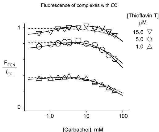
FIGURE 5: Determination of carbachol binding constants with carbamoylated AChE from the fluorescence of AChE-bound thioflavin T after the carbachol reactions have reached a final steady state. F_{ECN} values from mixtures of AChE (70–155 nM), thioflavin T (1.0–15.6 \mu M, as noted), and the indicated concentration of carbachol were determined from stopped-flow traces as in Figure 3. The F_{ECN} and then F_{ECN}/f_{ECL} data were analyzed with eq 11 as described for F_{EM} and then F_{EM}/f_{EL} in Figure 4. Parameters obtained from the data fitting are shown in Table 2. The dotted lines show the fit when carbachol is assumed to bind to only one site, (e.g., carbachol and thioflavin T compete for the P-site: (i_{EC}K_{ECS})^{-1} and i_{EC2}^{-1} fixed at 0 with fitted K_{M+S} = 57 ).
